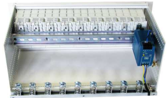
Stattox 502/503 19" Rack backside
