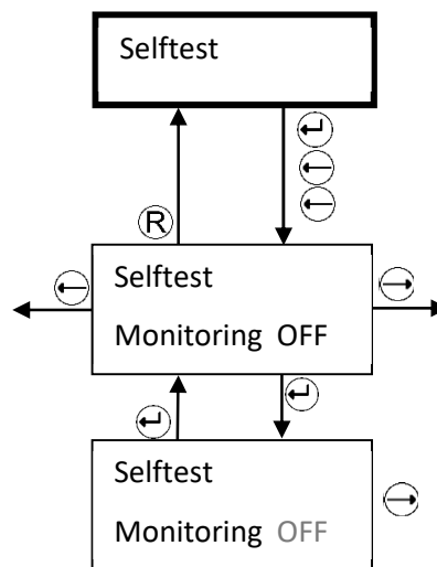
Picture 18: Submenu "Selftest - Monitoring off"
